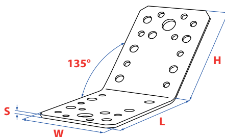
Merging square - 135°
