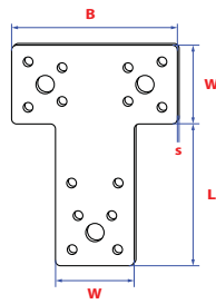
T-ridge large
