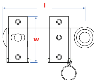
Kick-over latch
