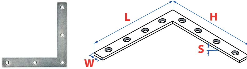
Raamhoek - 90°
