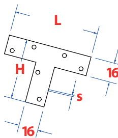
T-ridge
