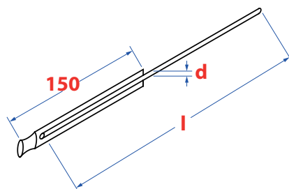
Slip tie
