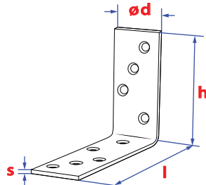
Frame connector
