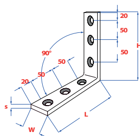
Cornice bracket - 90°
