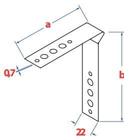
Spring anchor
